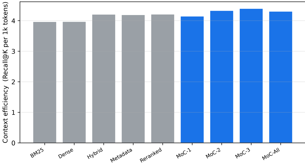
Context efficiency (mixed test split)
