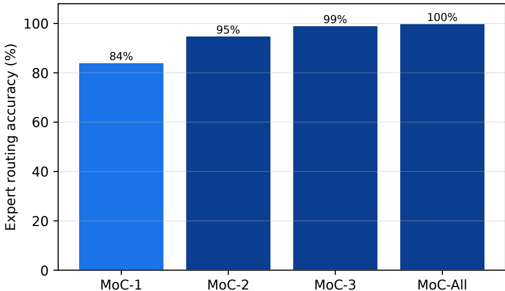
Routing accuracy by MoC-RAG variant
