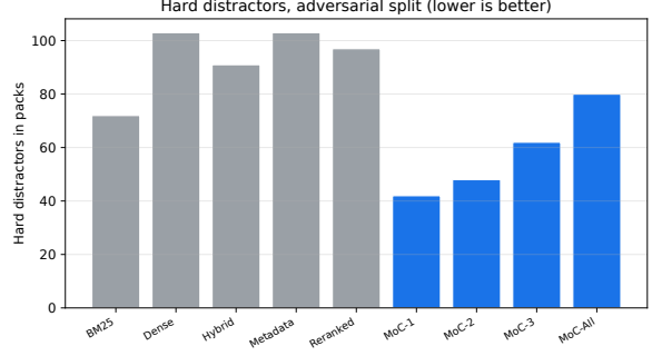
Figure 4: Hard distractors packed on the adversarial split (lower is better).
