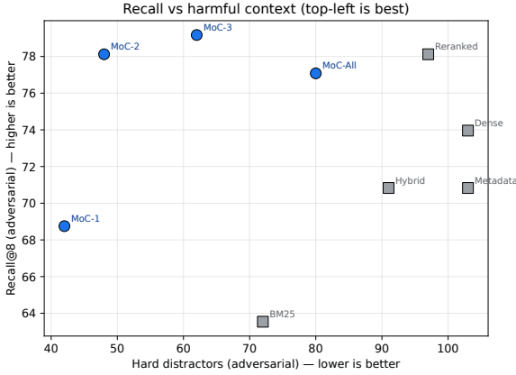
Figure 5: Pareto front: adversarial recall vs. hard distractors.
