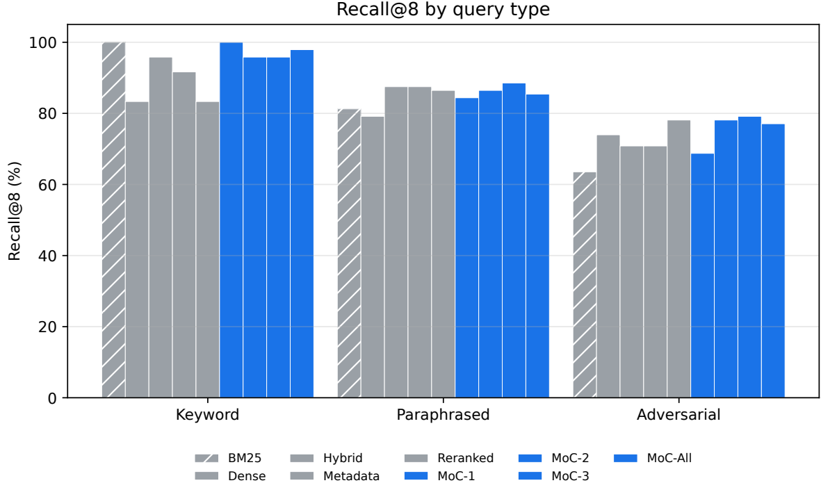
Figure 1: Recall@8 by query type (sentence-transformers embedder). BM25 leads on keyword-aligned queries but collapses under adversarial phrasing; MoC-RAG variants hold and overtake it on the adversarial split.
