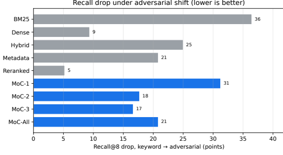
Figure 3: Recall@8 drop, keyword→adversarial (lower is better).
