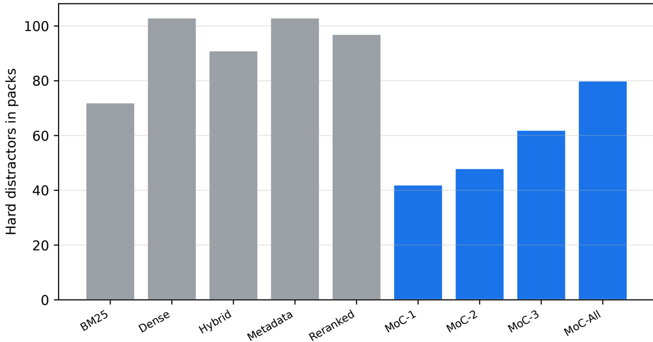
Hard distractors, adversarial split (lower is better)
