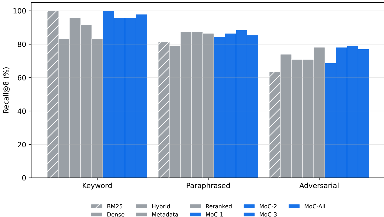
Recall@8 by query type
