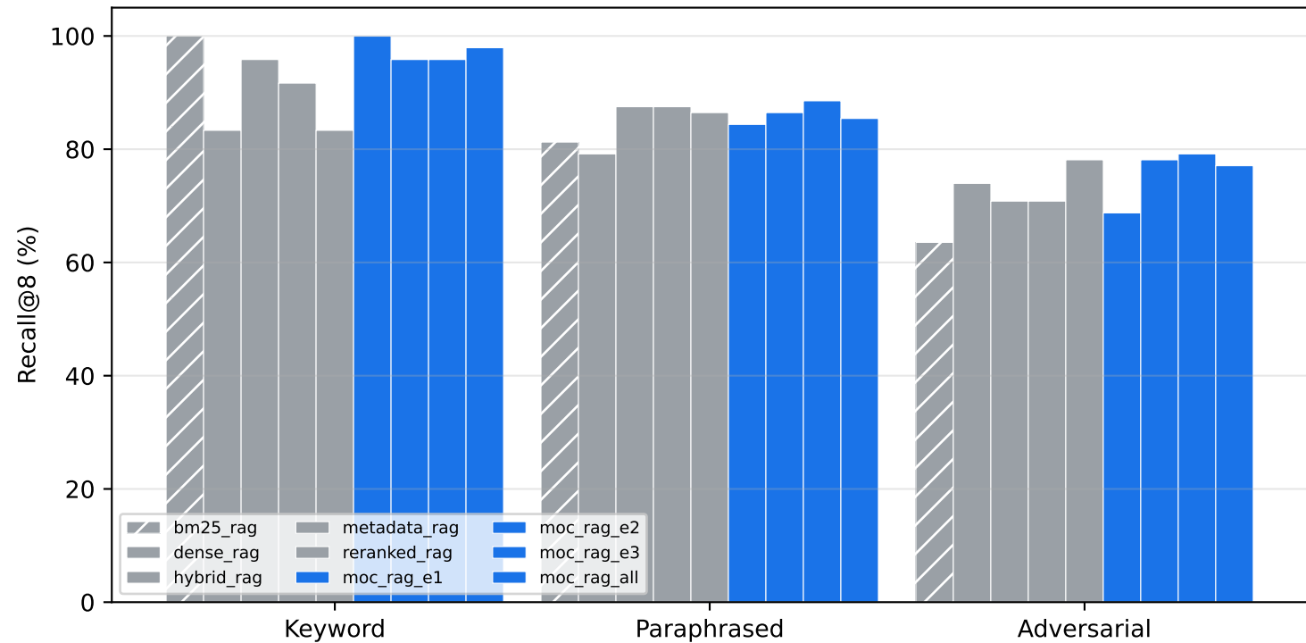
Recall by query type — BM25 collapses on adversarial; MoC-RAG holds
