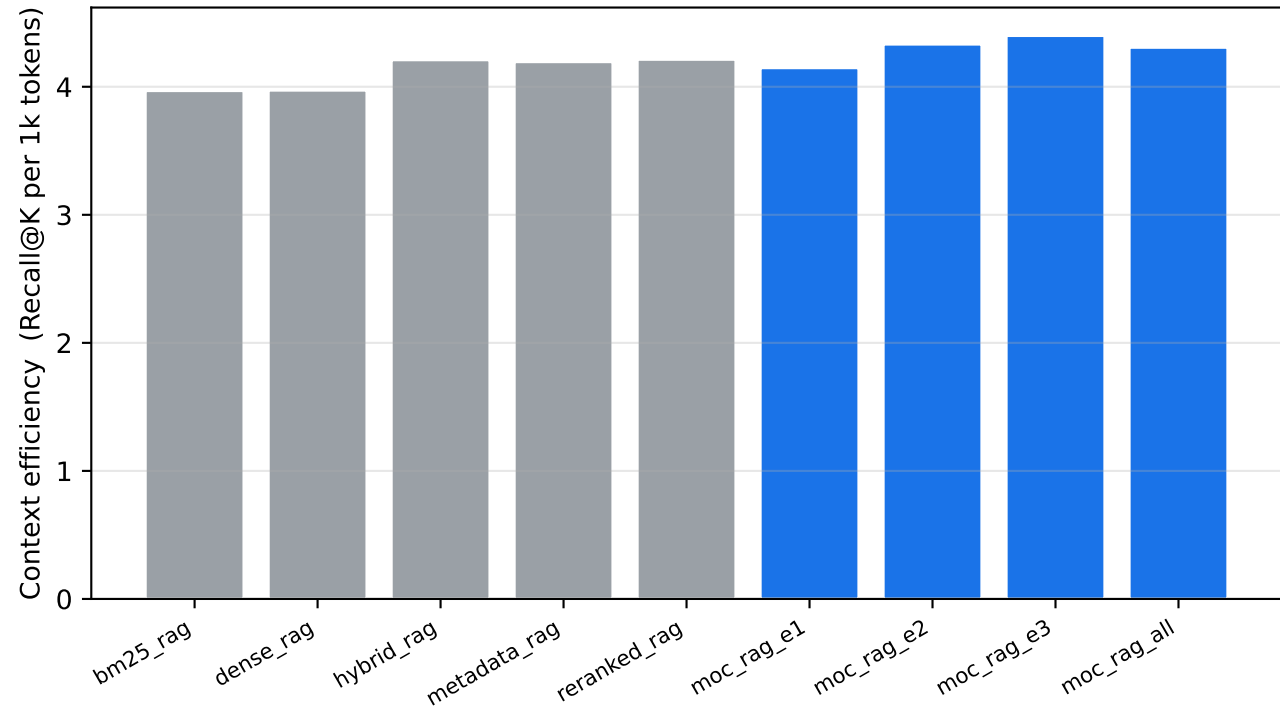
Context efficiency by method (mixed test split)
