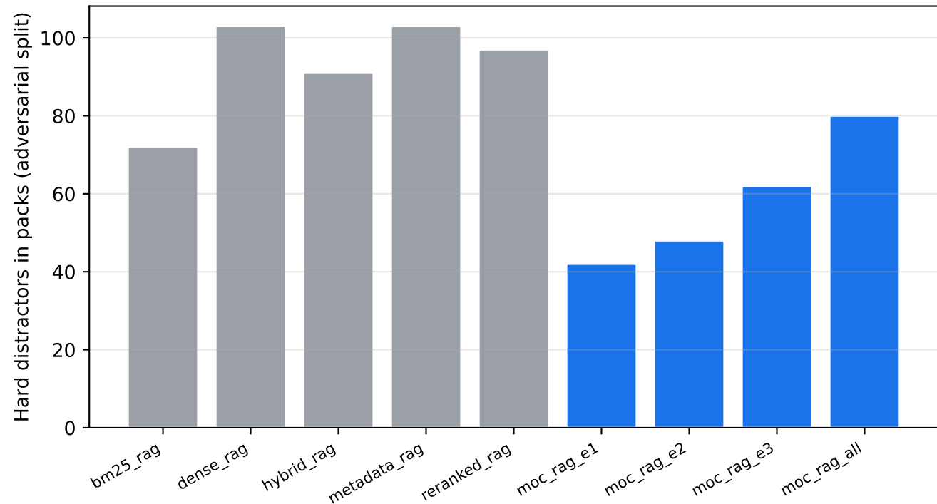
Harmful context packed — MoC-RAG carries ~half the dense family
