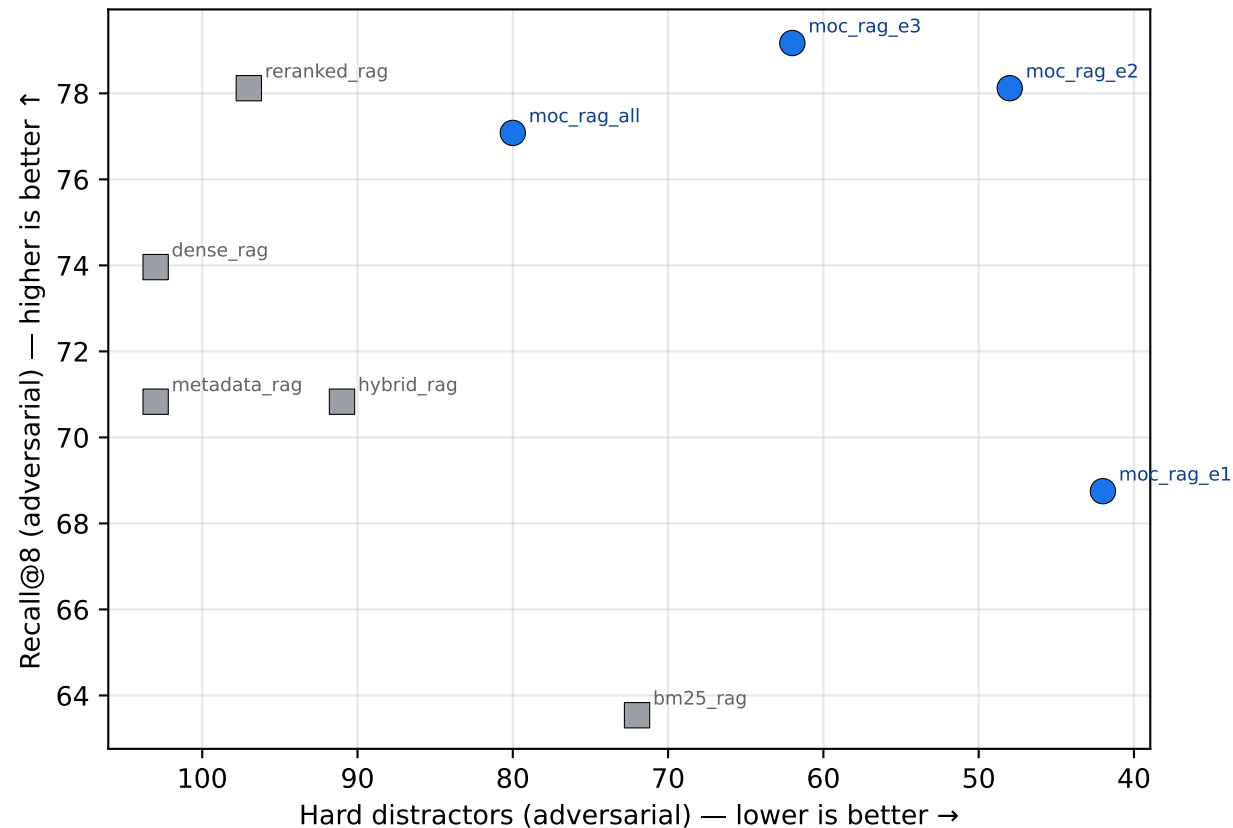
Pareto front: adversarial recall vs harmful context (top-right is best; MoC-RAG dominates the dense family)
