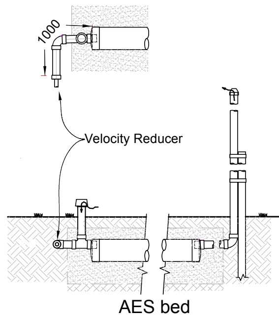
VV Venting with Velocity Reducer
