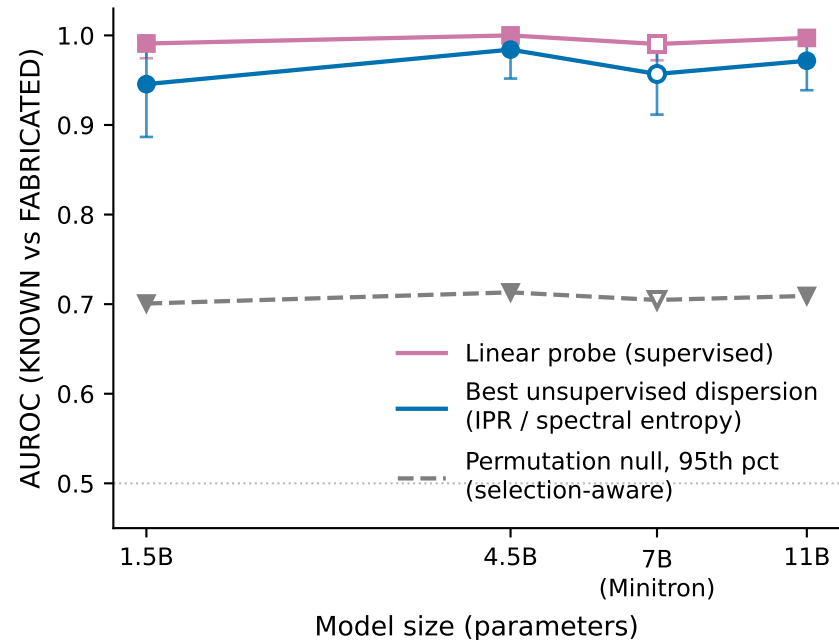
(a) Activation signal — saturated at all scales
