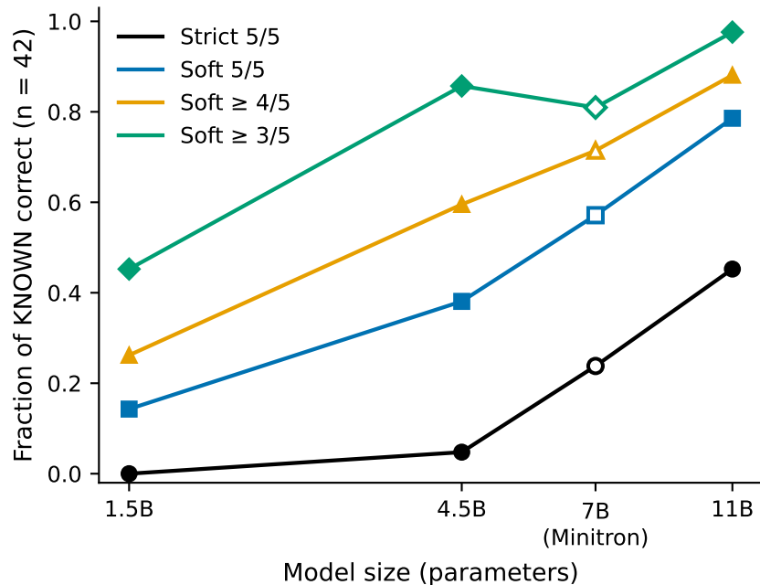
(b) Behavioral correctness — rises with scale
