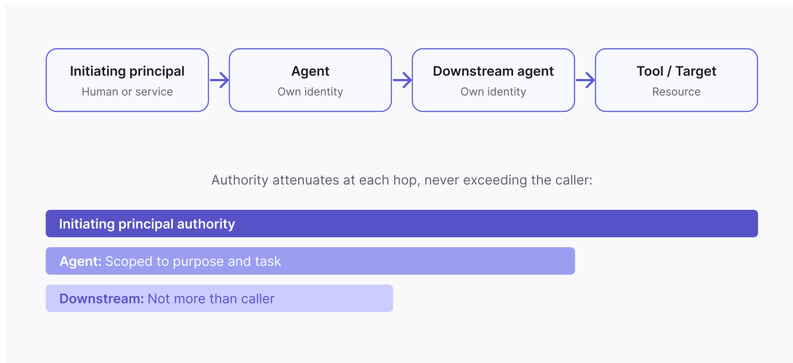
Figure 5 Authority attenuating along the chain: initiating principal, agent, downstream agent, tool or target - each hop scoped no wider than its caller.
