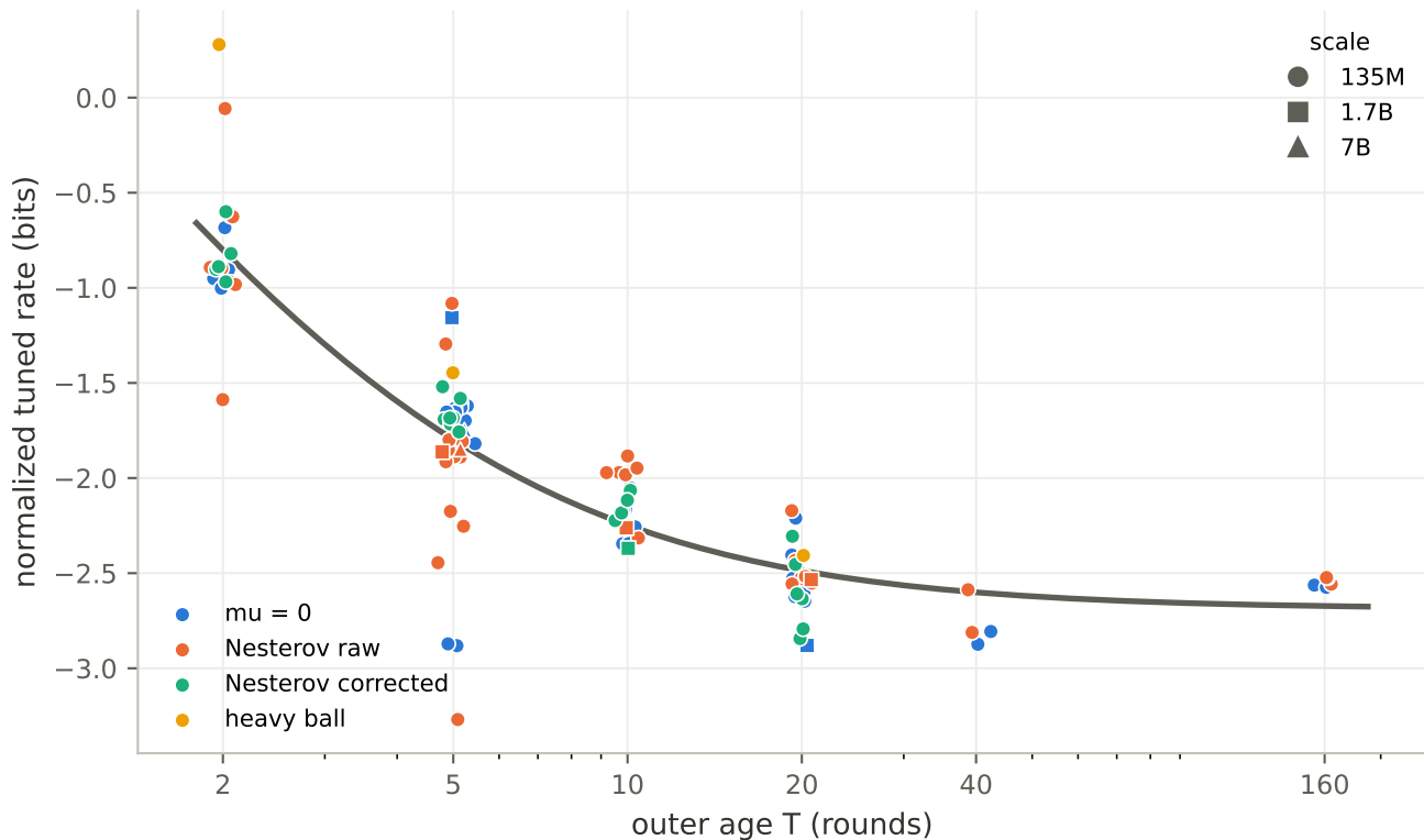
H7-rho-floor-S collapse: \log_2 \eta^* minus scale/kinematic/convention/S terms line = \log_2(T^{-\alpha} + f) , \alpha=1.256 , f=0.155
