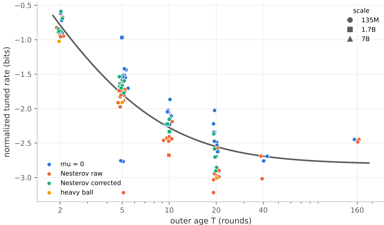
C1sat-H7kin collapse: \log_2 \eta^* minus scale/kinematic/convention/S terms kinematics = theorem T/C; line = \log_2(T^{-\alpha} + f) , \alpha=1.195 , f=0.143
