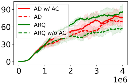
Breakout
