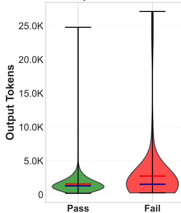
OpenAI Codex
