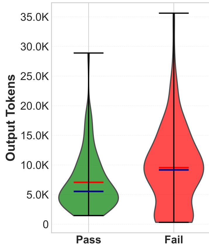
Qwen Code
