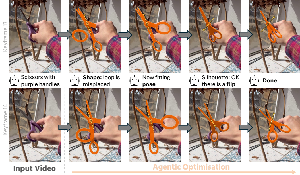
Figure 2: Method. Given an input video (left), our agentic optimisation loop iteratively refines the shape and pose of the observed object (right). The middle panels summarise the agent’s reasoning throughout the optimisation process. Our harness provides the VLM with numerical optimisation tools for precise pose fitting, together with temporal diagnostics for assessing consistency across keyframes. The final output is a reconstructed object model together with its estimated generalised pose at every observed keyframe.
