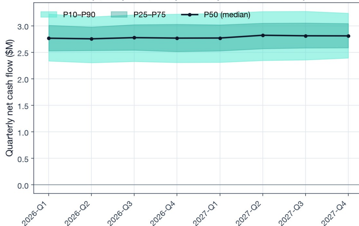
Portfolio Net Cash-Flow Forecast — Monte Carlo Confidence Bands (1,000 paths, independent paths*, base case)
