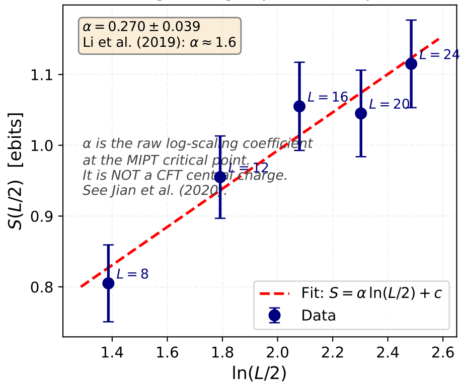
Log Scaling at p = 0.160 \approx p_c
