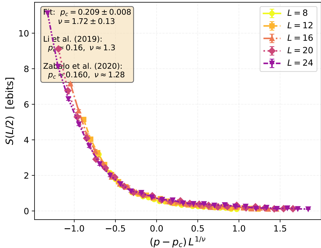
FSS Collapse: p_c = 0.209 , \nu = 1.72
