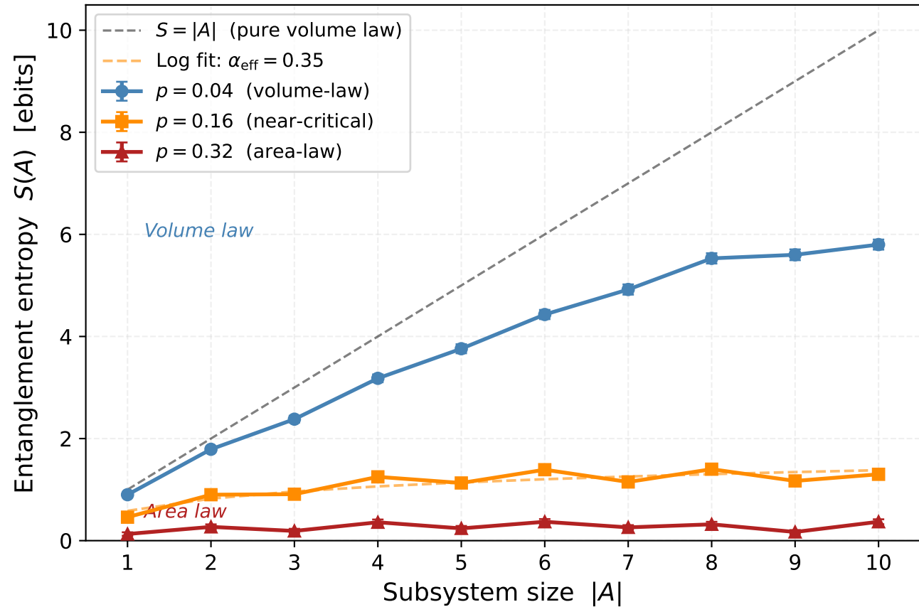
Entanglement Profile S(A) vs |A| ( L = 20, 100 samples)
