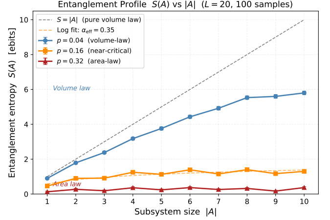
FIG. 5. Entanglement profile S(A) vs. subsystem size |A| for L = 20 (100 disorder realizations; shaded bands: \pm 1 SEM). The contiguous subsystem A = \{0, \dots, |A| - 1\} . Three representative rates are shown: p = 0.04 (volume-law phase), p = 0.16 (near the thermodynamic p_c ), and p = 0.32 (area-law phase). The dashed black line S = |A| marks the pure volume-law reference. In the volume-law phase the profile grows roughly linearly with |A| ; in the area-law phase it is approximately flat; near p_c the growth is sublinear. The orange dashed curve shows a log fit S = \alpha_{\text{eff}} \ln |A| + c to the p = 0.16 data ( \alpha_{\text{eff}} \approx 0.35 ; the small value is expected at L = 20 as discussed in Sec. ).
