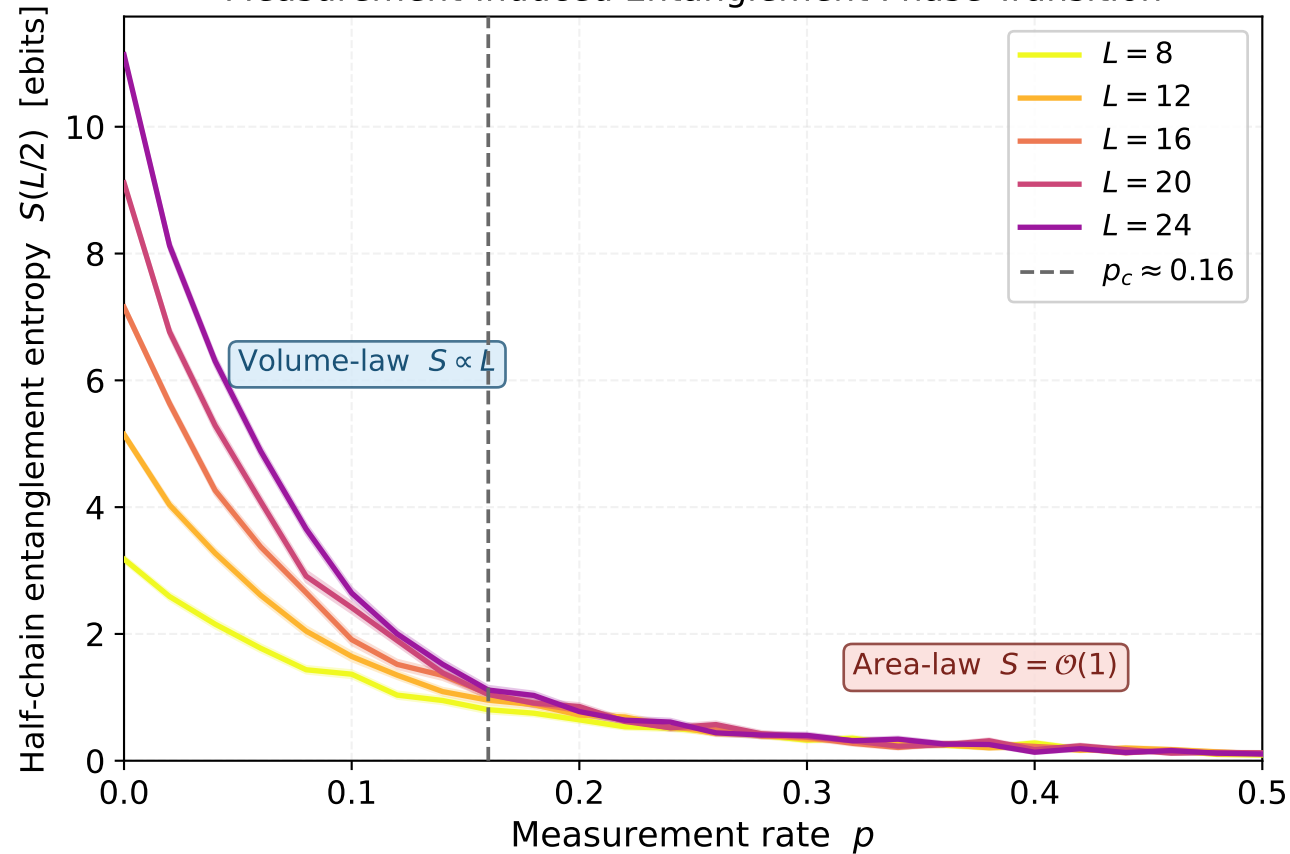
Measurement-Induced Entanglement Phase Transition
