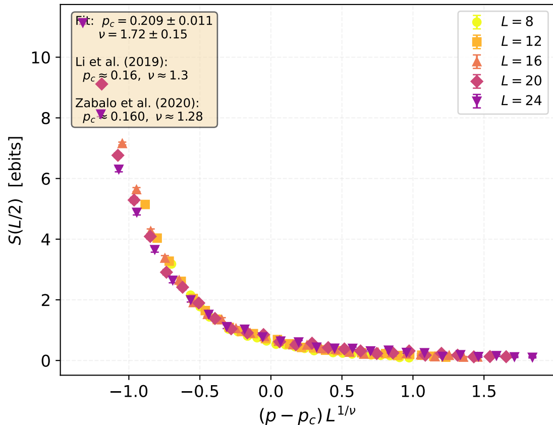
FSS Collapse: p_c = 0.209 , \nu = 1.72
