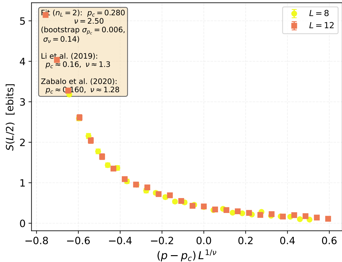
FSS Collapse: p_c = 0.280 , \nu = 2.50
