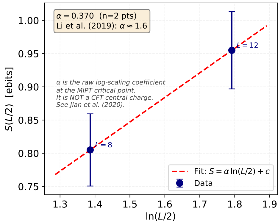
Log Scaling at p = 0.160 \approx p_c
