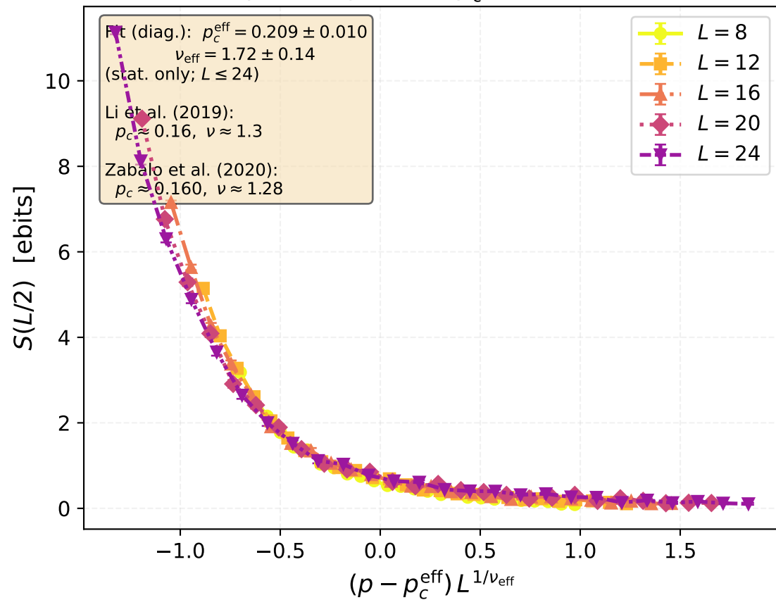
FSS Collapse (diagnostic): p_c^{\text{eff}} = 0.209 , \nu_{\text{eff}} = 1.72
