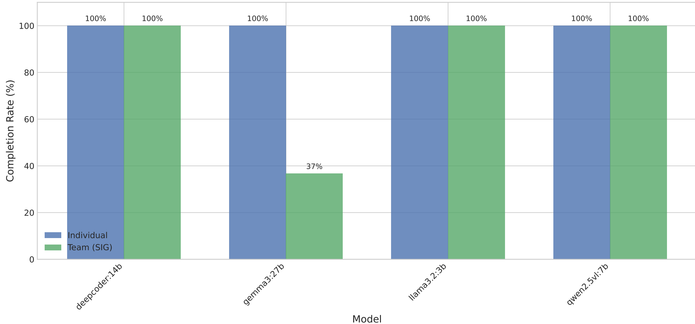
Session Completion Rate by Mode and Model
