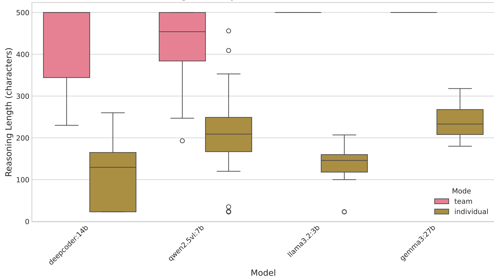
Reasoning Verbosity: Team (SIG) vs Individual Mode
