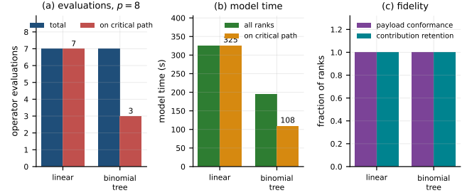
Figure 5: Semantic reduction over eight Cursor subagents. The two schedules perform the same number of model evaluations of the operator; only the tree takes them off the root’s critical path, cutting critical-path model time 3.0× with identical coverage. Elapsed time is not shown because it is dominated by executor admission rather than by the schedule.
