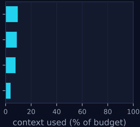
context pressure
