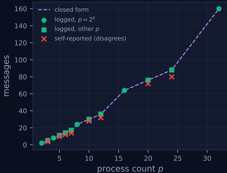
allreduce/recursive_doubling: messages
