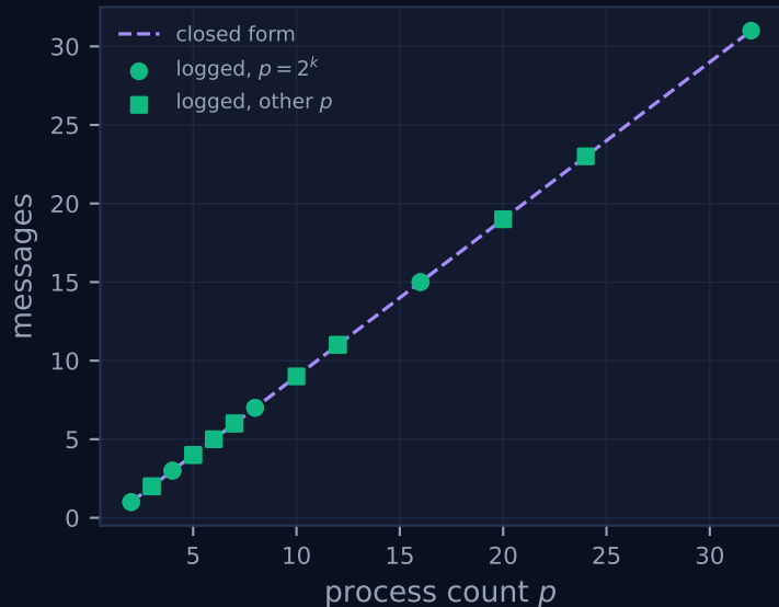
scatter/binomial: messages
