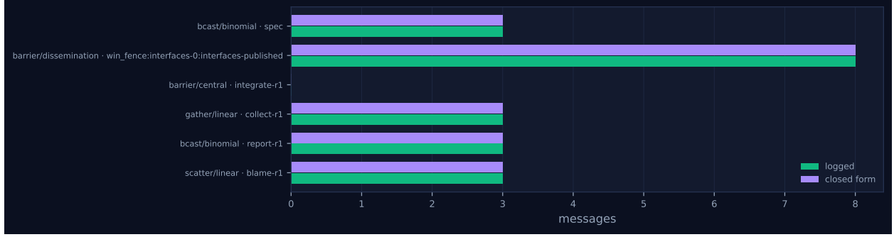
Figure 3: Logged message count against the closed-form prediction, per invocation. A red diamond marks a disagreement between the implementation and its own cost model.
