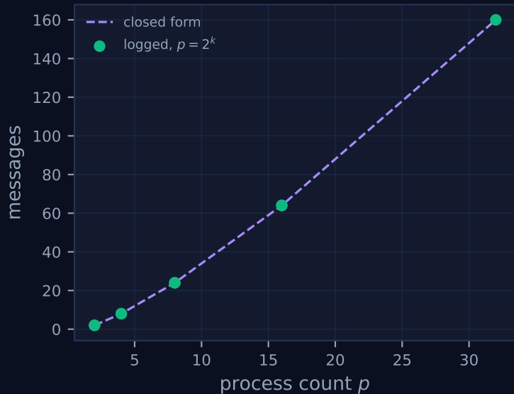
allgather/recursive_doubling: messages
