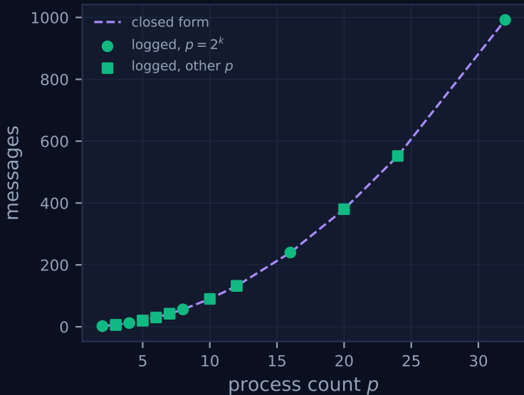
allgather/ring: messages
