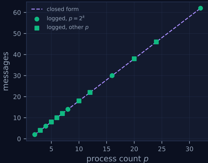
allreduce/reduce_bcast: messages
