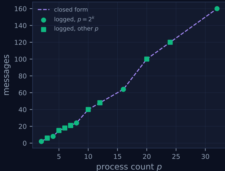
alltoall/bruck: messages
