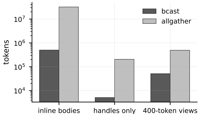
(a) total tokens into all contexts
