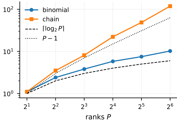
(a) critical path, agent operator
