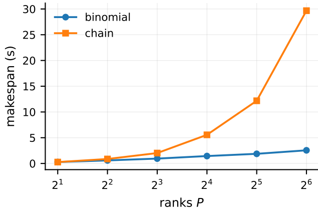
(b) makespan, 0.25s per application
