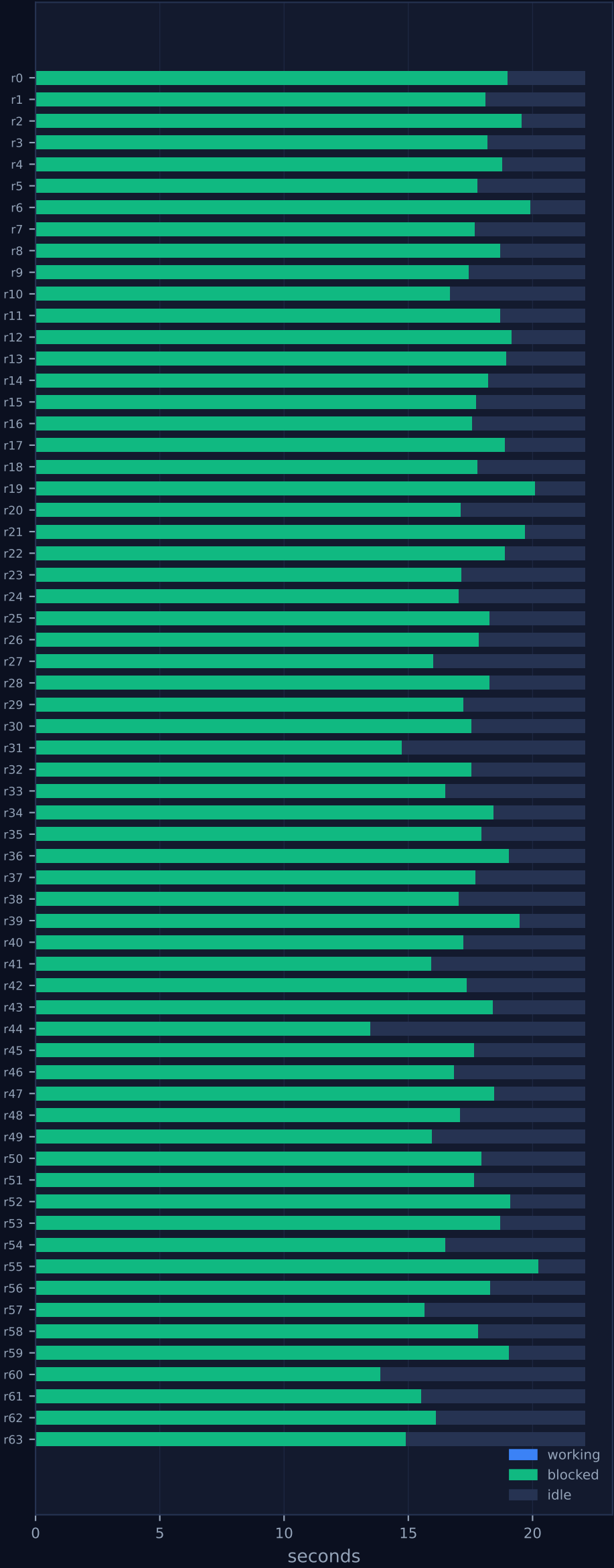
where each rank's wall clock went
