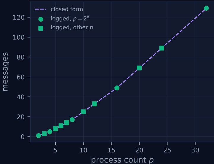
scan/recurse_doubling: messages
