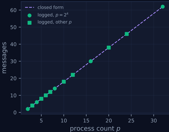
allreduce/reduce_bcast: messages
