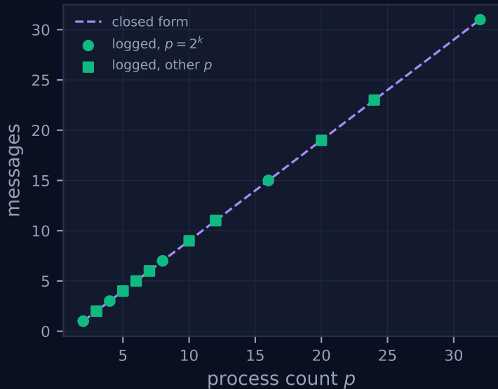
reduce/chain: messages
