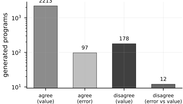
(a) 2500 programs, 92.4% agree
