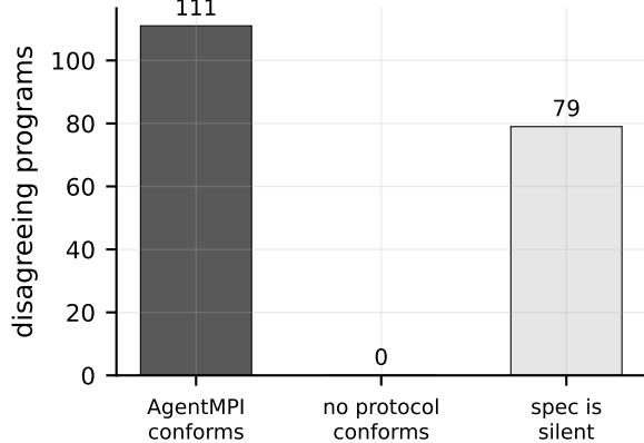
(b) attribution (1 root cause)
