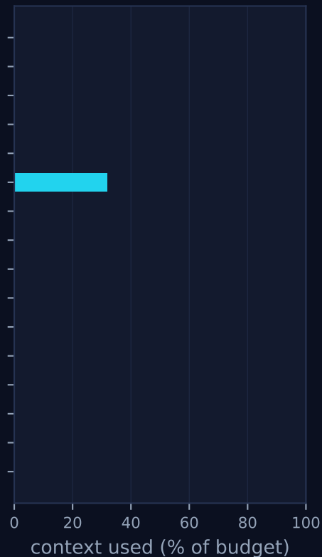
context pressure
