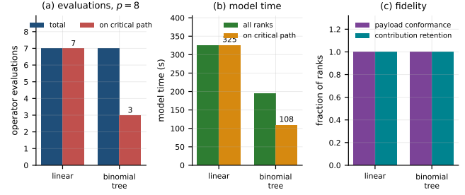
Figure 5: Semantic reduction over eight Cursor subagents. The two schedules perform the same number of model evaluations of the operator; only the tree takes them off the root’s critical path, cutting critical-path model time 3.0× with identical coverage. Elapsed time is not shown because it is dominated by executor admission rather than by the schedule.
