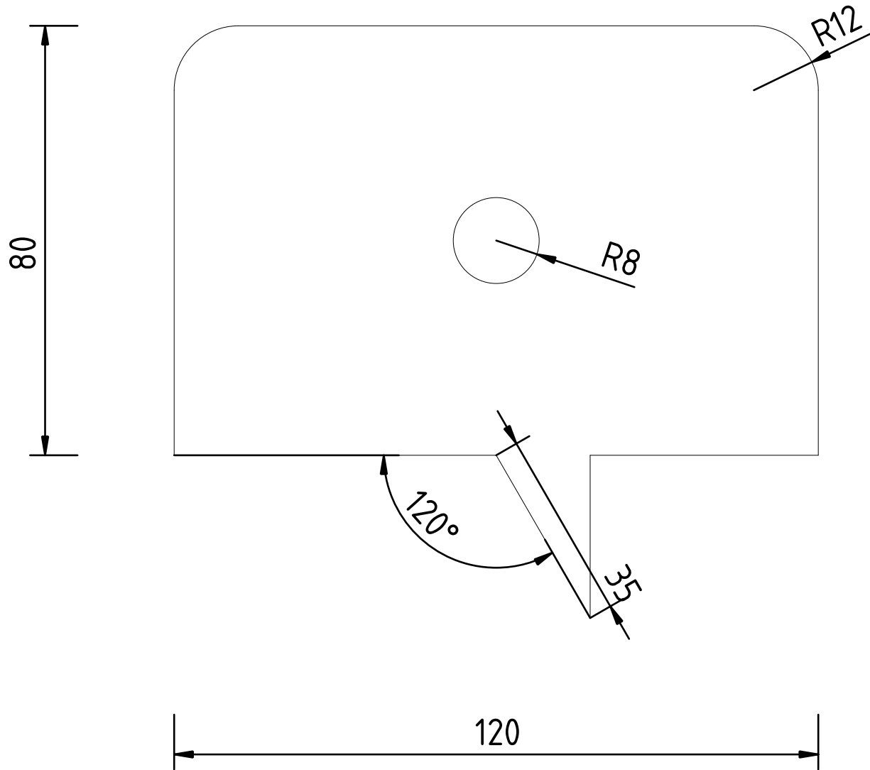
Material: Steel, 3mm Mounting Bracket
