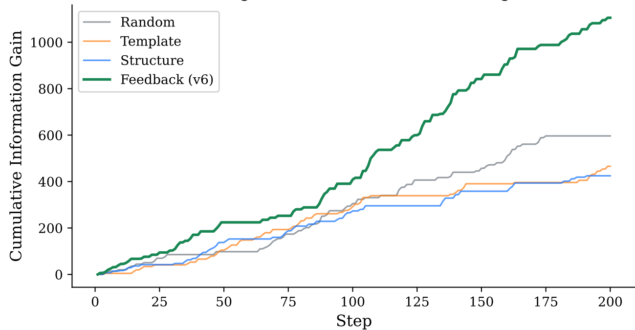
Learning Rate Across Question Strategies
