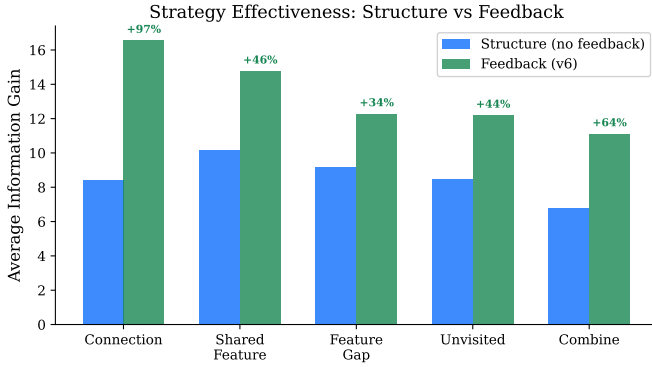
Fig. 3. Average information gain per strategy: structure mode (equal weights) vs. feedback mode (learned weights). Every strategy improves with feedback.
