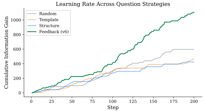
Fig. 2. Cumulative information gain over 200 steps. Feedback mode accelerates after step ~40.
