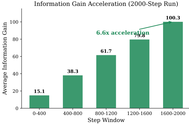
Fig. 4. Average information gain per 400-step window across 2000 steps. IG accelerates rather than plateaus as the knowledge graph densifies.
