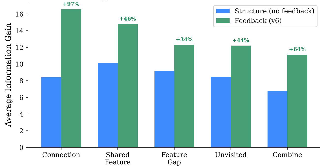
Strategy Effectiveness: Structure vs Feedback
